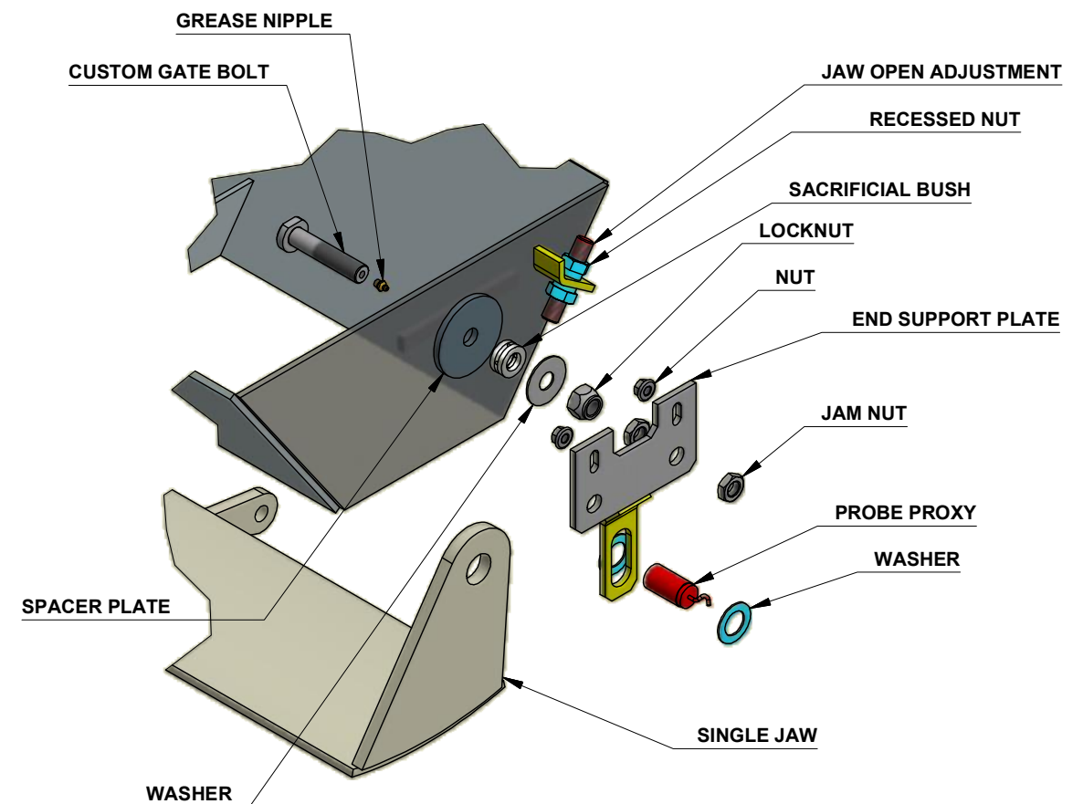
SINGLE JAW GATE
